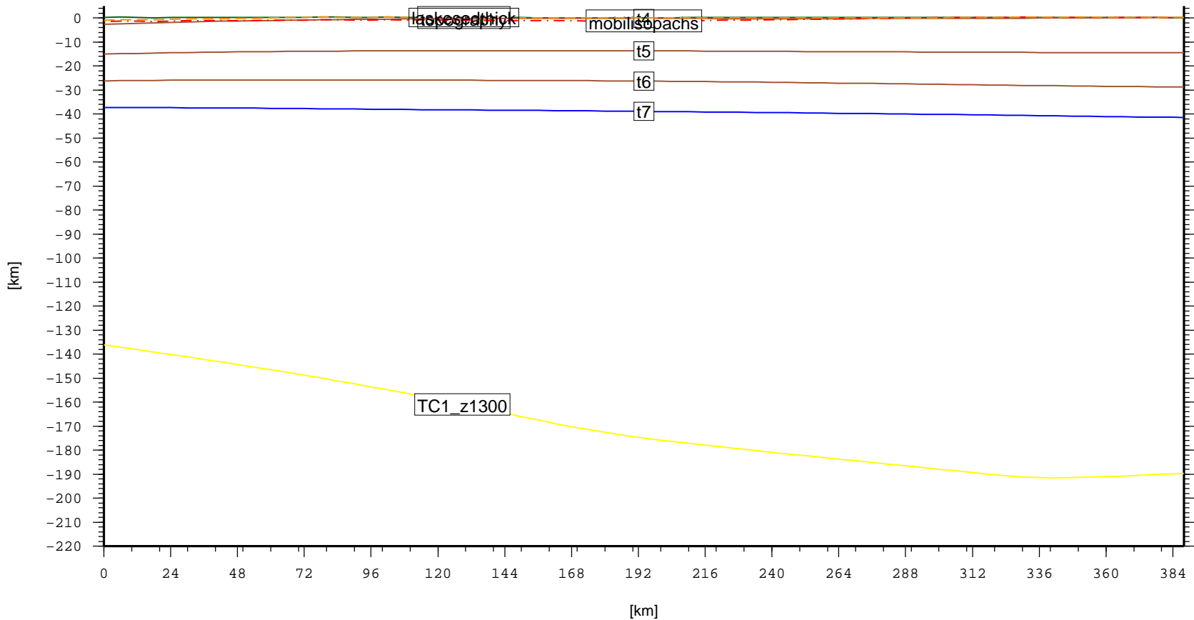
Cross section – AFR.BidaBasin (topo, laske sedthick, t4, t5, t6, t7)
