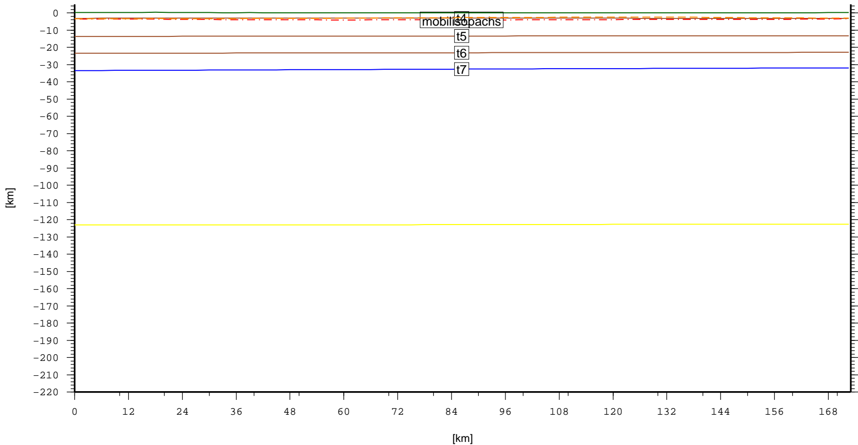
Cross section – AFR.GindiBasin (topo, laske sedthick, t4, t5, t6, t7)
