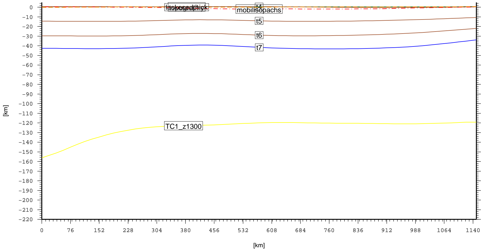
Cross section – AFR.KhartoumBasin (topo, laske sedthick, t4, t5, t6, t7)
