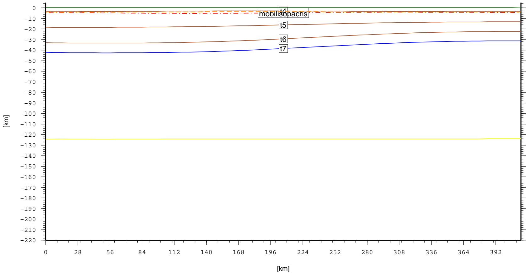
Cross section – AFR.MarmaricaBasin (topo, laske sedthick, t4, t5, t6, t7)
