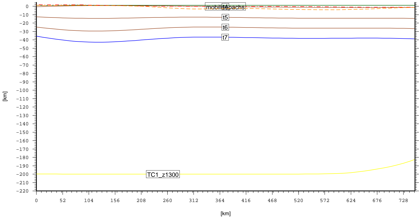
Cross section – AFR.OwamboBasin (topo, laske sedthick, t4, t5, t6, t7)
