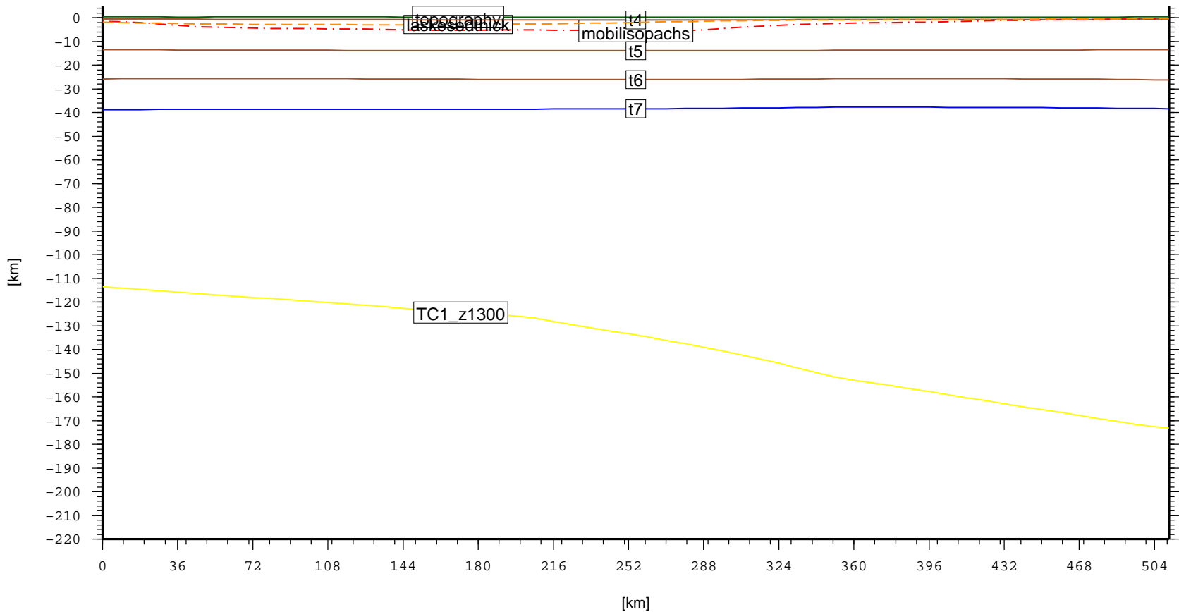
Cross section – AFR.RegganeBasin (topo, laske sedthick, t4, t5, t6, t7)
