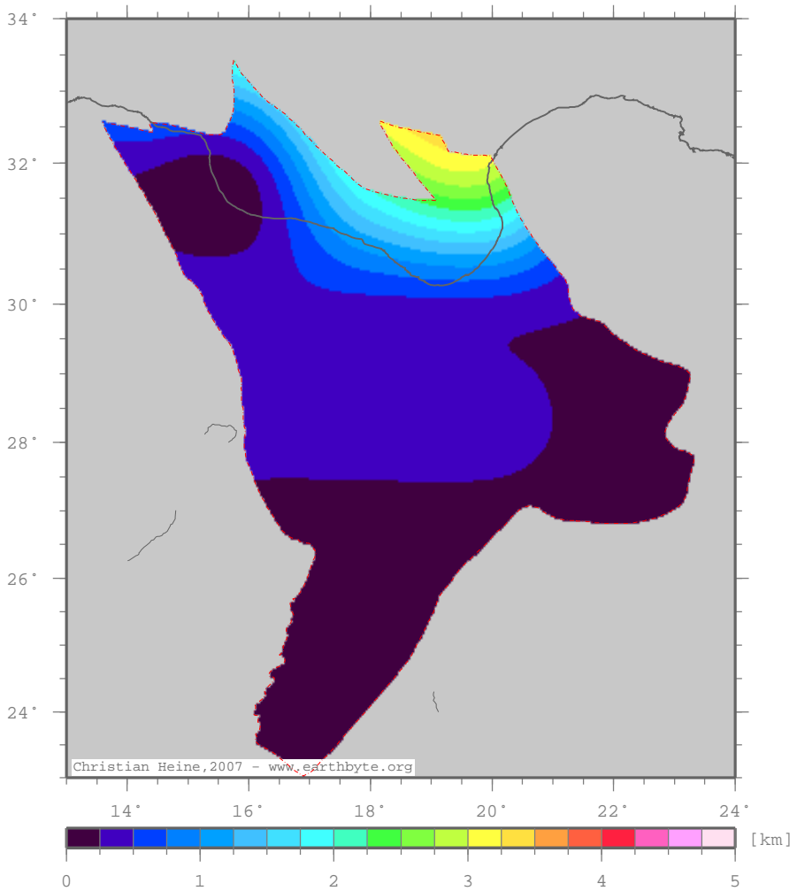
Total tectonic subsidence
