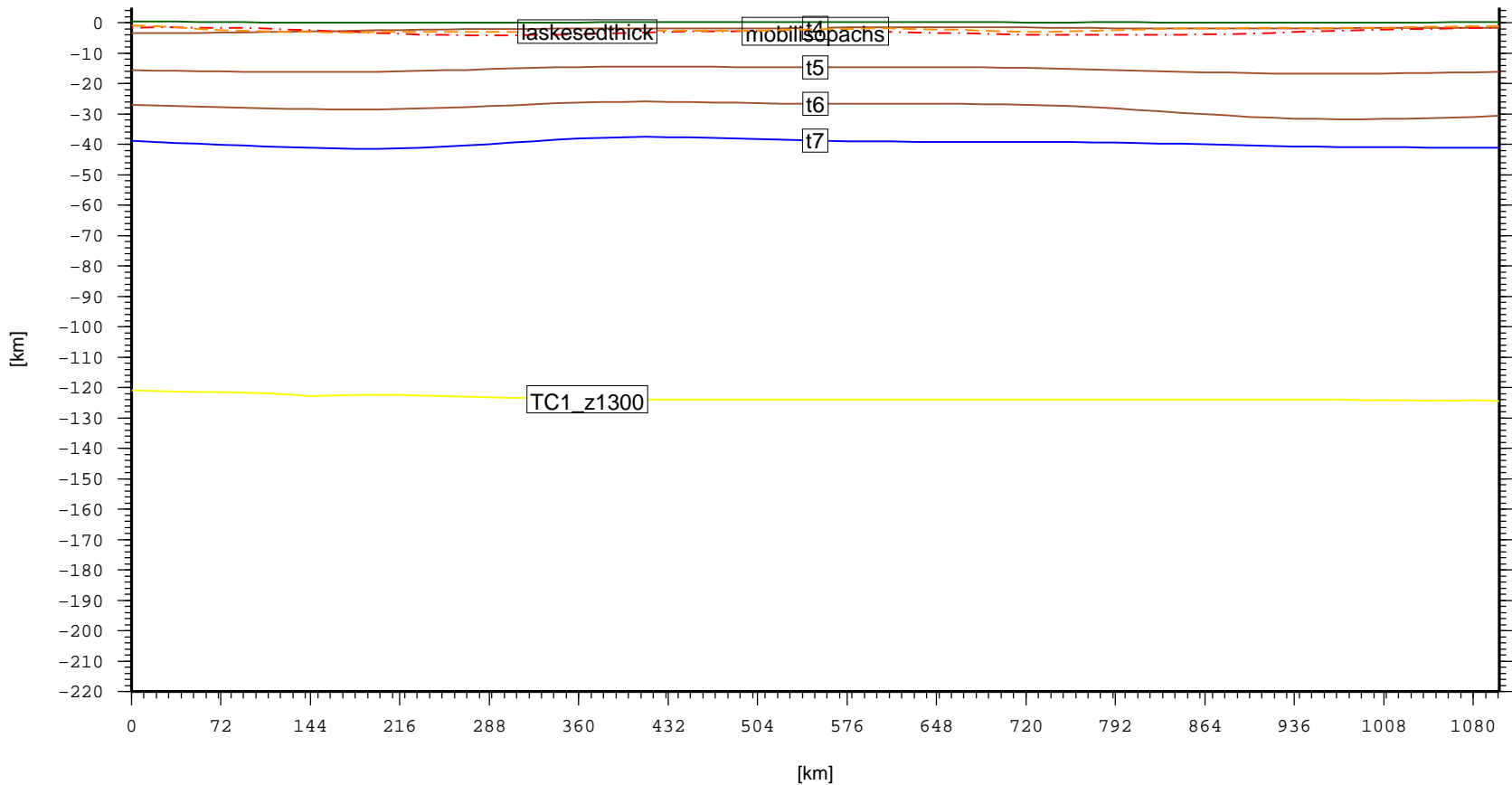
Cross section – AFR.SirteBasin (topo, laske sedthick, t4, t5, t6, t7)
