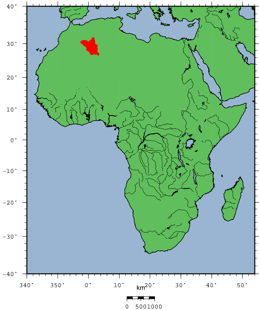
Location map AFR.TimimounBasin.
