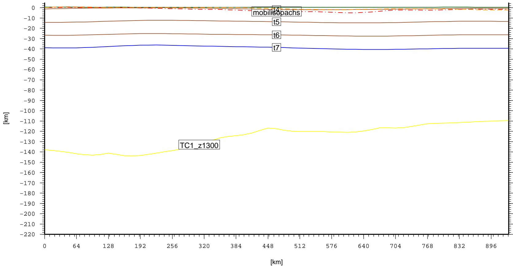
Cross section – AFR.TindoufBasin (topo, laske sedthick, t4, t5, t6, t7)
