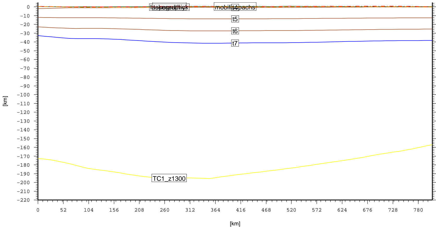
Cross section – AFR.VoltaianBasin (topo, laske sedthick, t4, t5, t6, t7)
