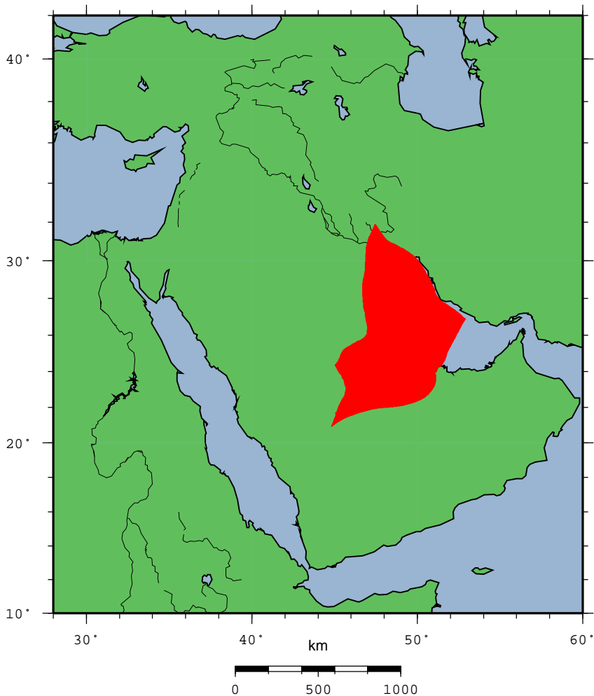
Location map ARA.CentralArabianProvince_ArabianBasin.
