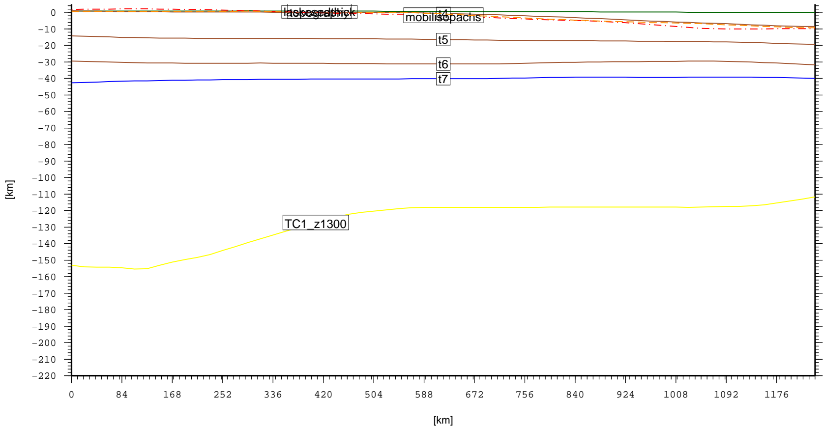
Cross section – ARA.CentralArabianProvince_ArabianBasin (topo, lasce sedthick, t4, t5, t6, t7)
