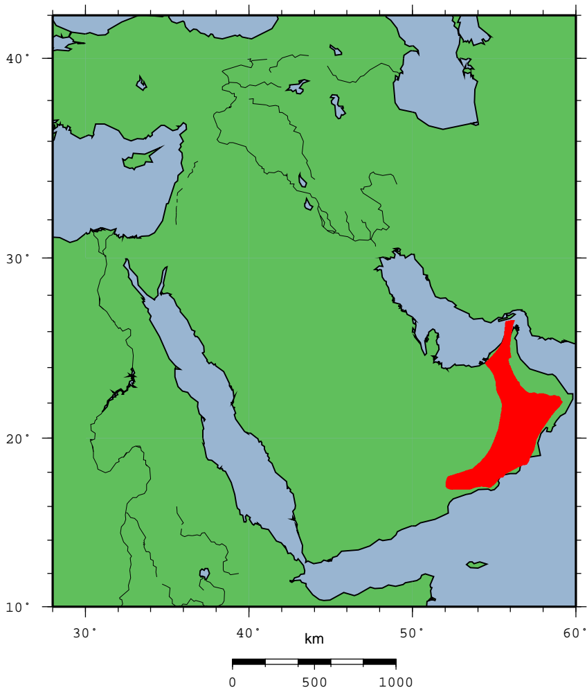
Location map ARA.OmanBasin.
