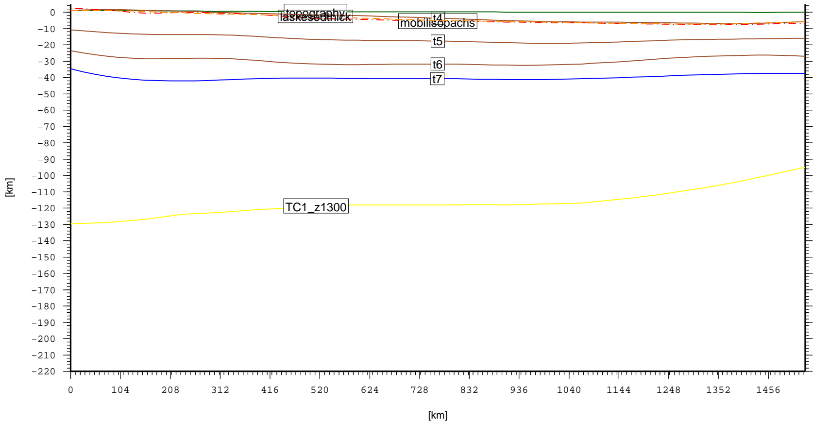
Cross section – ARA.Rub_AIKhaliProvince_ArabianBasin (topo, laske sedthick, t4, t5, t6, t7)
