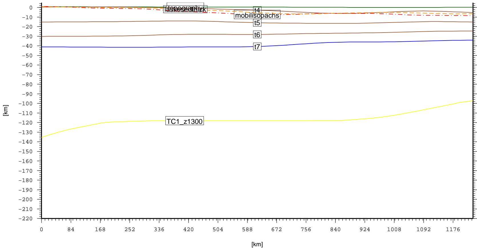
Cross section – ARA.Widyan–MesopotamiaProvince_ArabianBasin (topo, laske sedthick, t4, t5, t6, t7)
