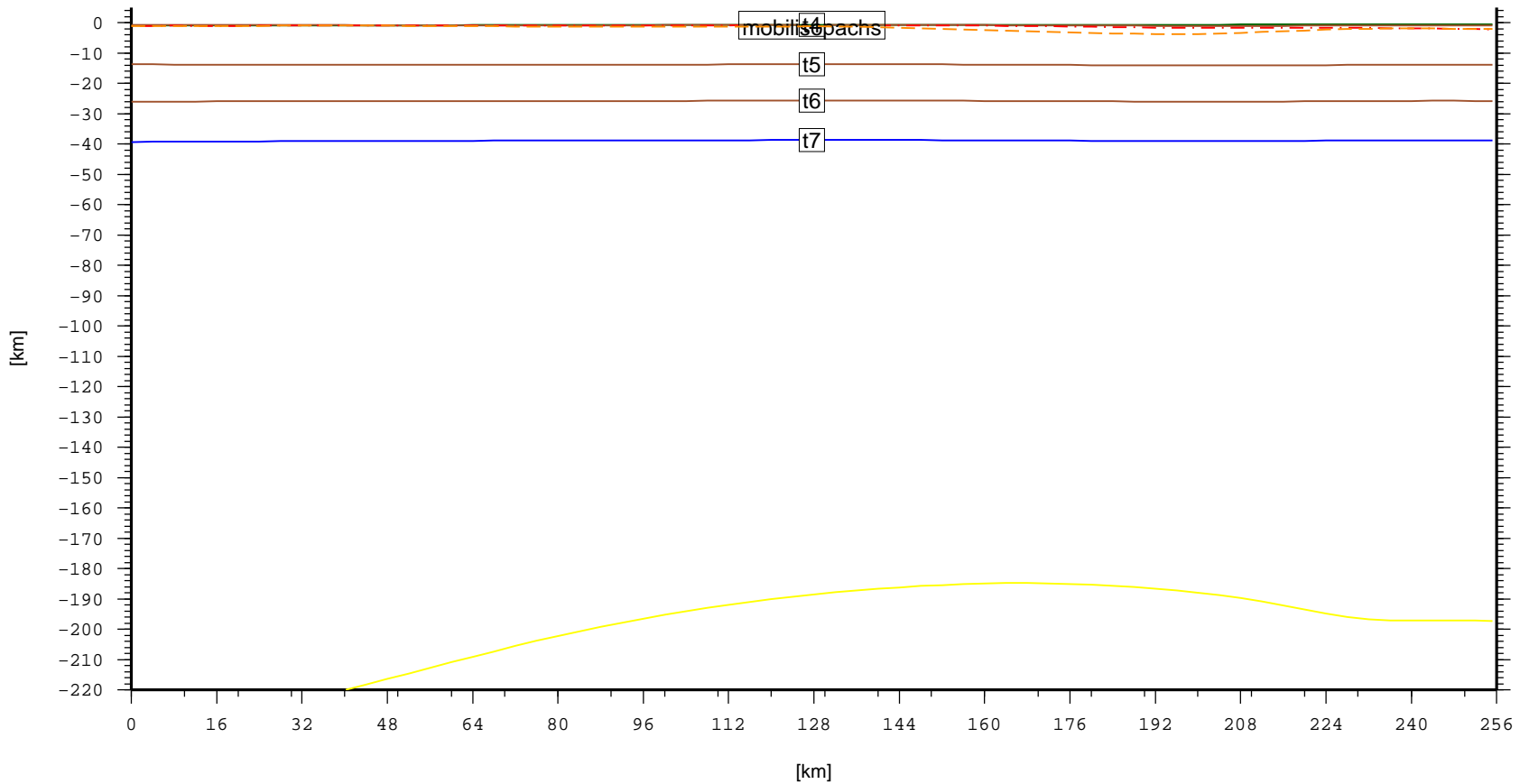
Cross section – ARC.LancasterBasin (topo, laske sedthick, t4, t5, t6, t7)
