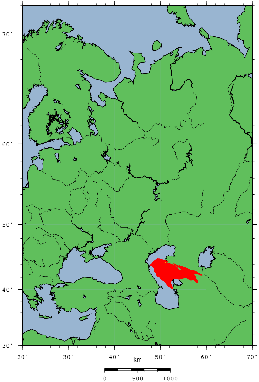
Location map CAS.MangyshlakBasin.
