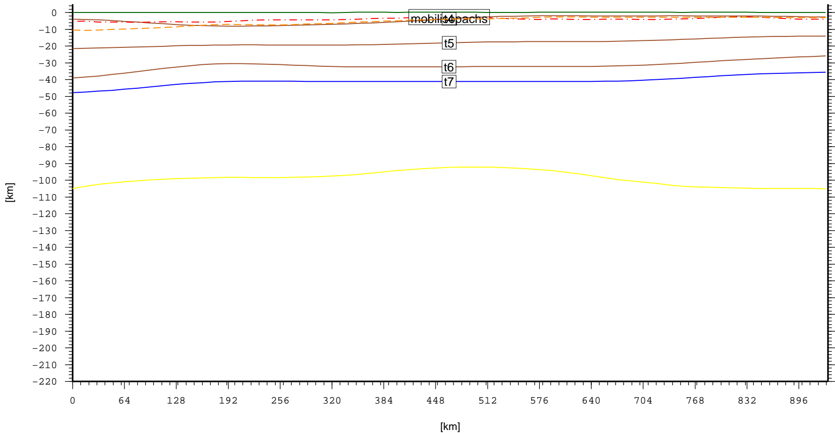
Cross section – CAS.MangyshlakBasin (topo, laske sedthick, t4, t5, t6, t7)
