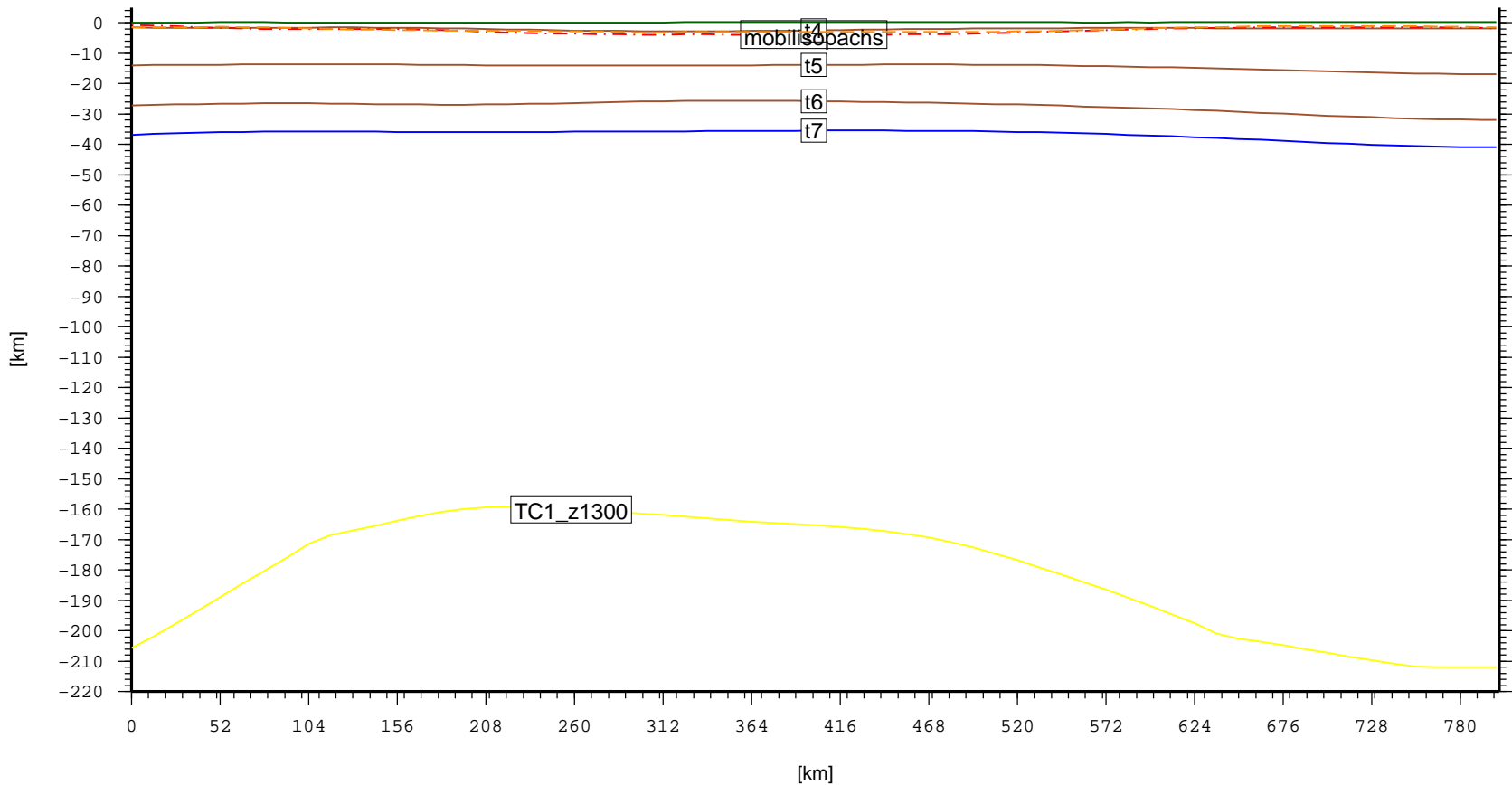
Cross section – CAS.MezenSyneclise (topo, laske sedthick, t4, t5, t6, t7)
