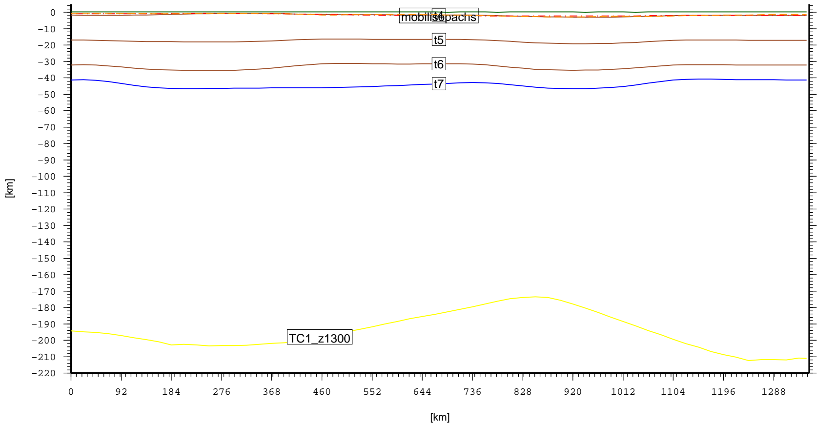
Cross section – CAS.MoscowBasin_Syneclise (topo, laske sedthick, t4, t5, t6, t7)
