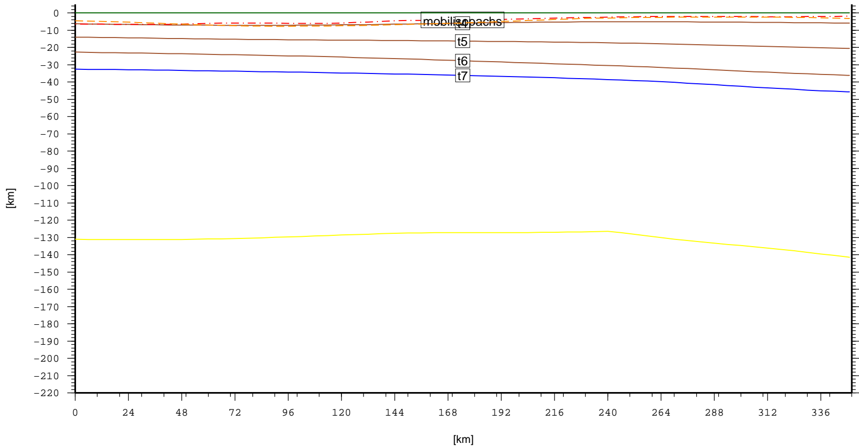
Cross section – CAS.NorthBlackSea–CrimeaBasin (topo, laske sedthick, t4, t5, t6, t7)
