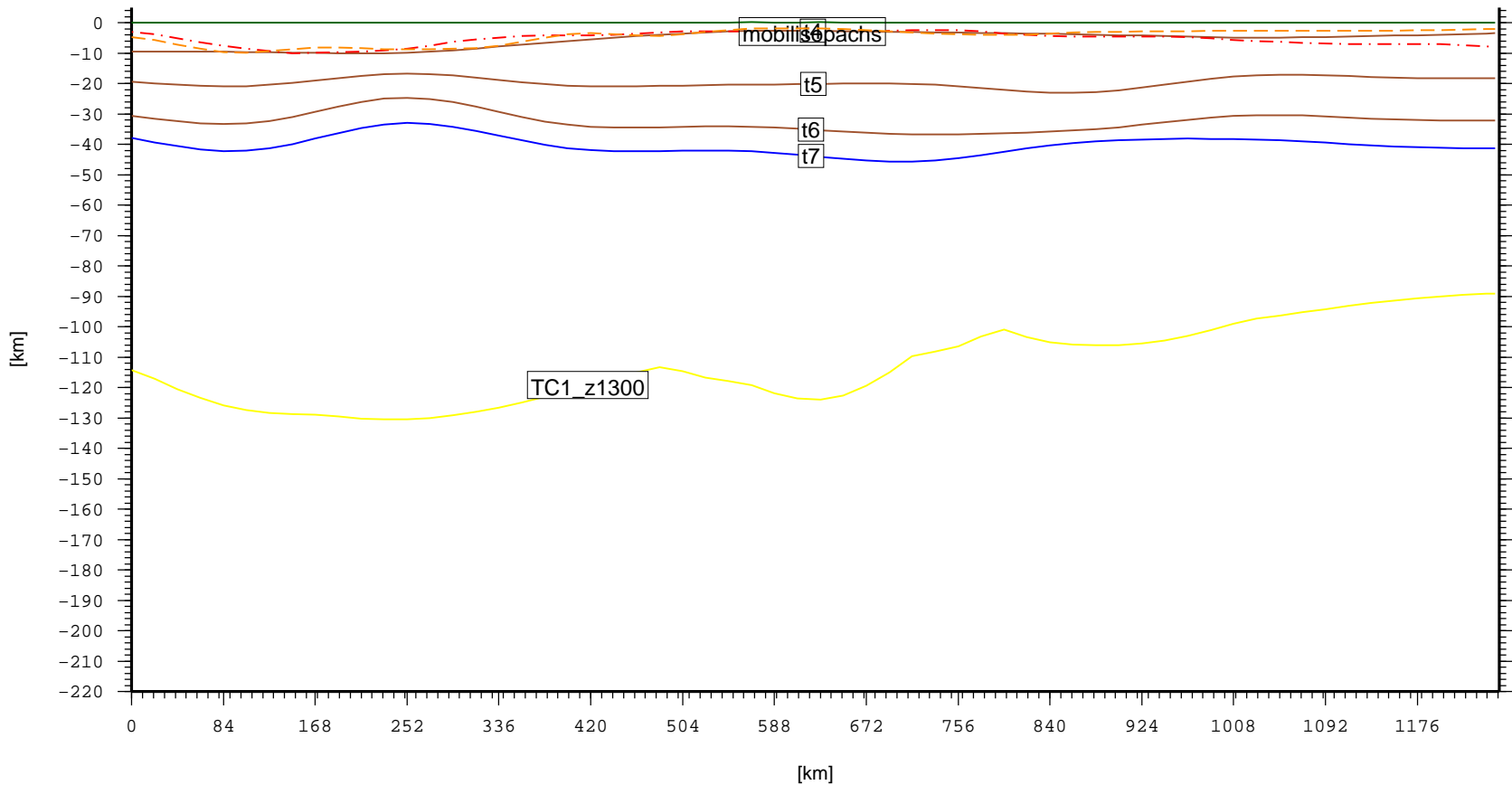
Cross section – CAS.NorthCaucasusPlatform (topo, laske sedthick, t4, t5, t6, t7)
