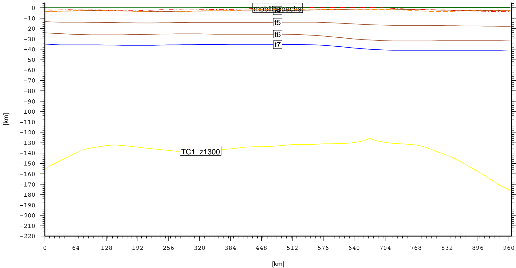
Cross section – CAS.Pre–TimanTrough (topo, laske sedthick, t4, t5, t6, t7)
