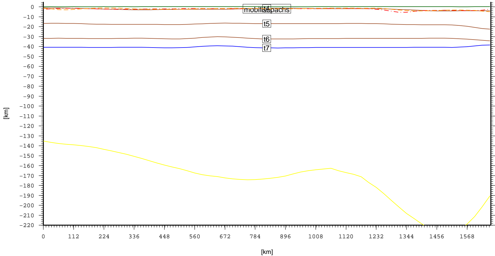
Cross section – CAS.Volga–UralBasin (topo, laske sedthick, t4, t5, t6, t7)
