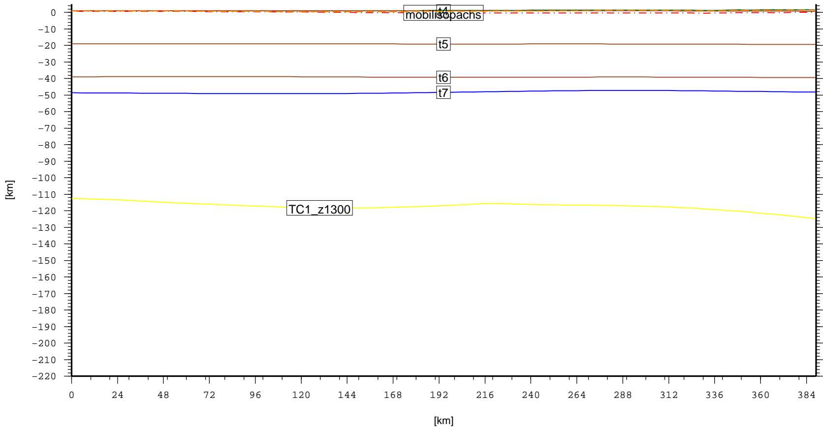
Cross section – CHN.EjinQiBasin (topo, laske sedthick, t4, t5, t6, t7)
