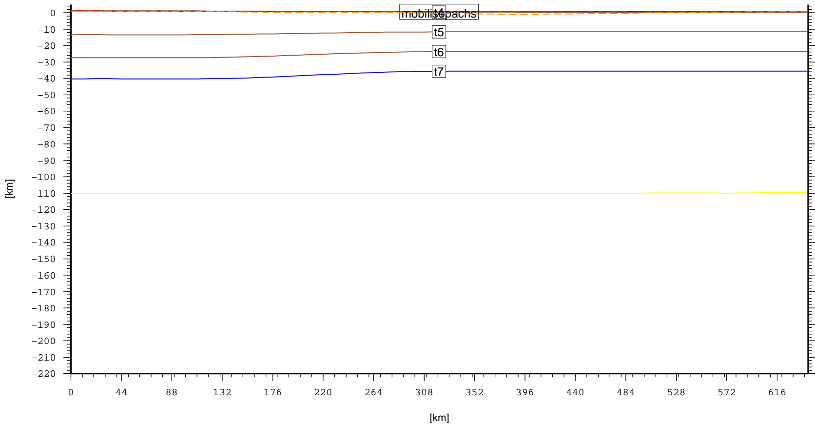
Cross section – CHN.Hailar_HulunchiBasin (topo, laske sedthick, t4, t5, t6, t7)
