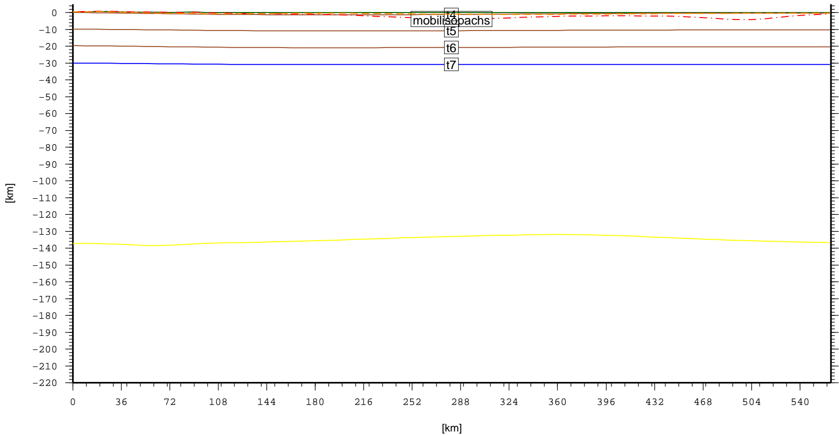
Cross section – CHN.HefeiBasin (topo, laske sedthick, t4, t5, t6, t7)
