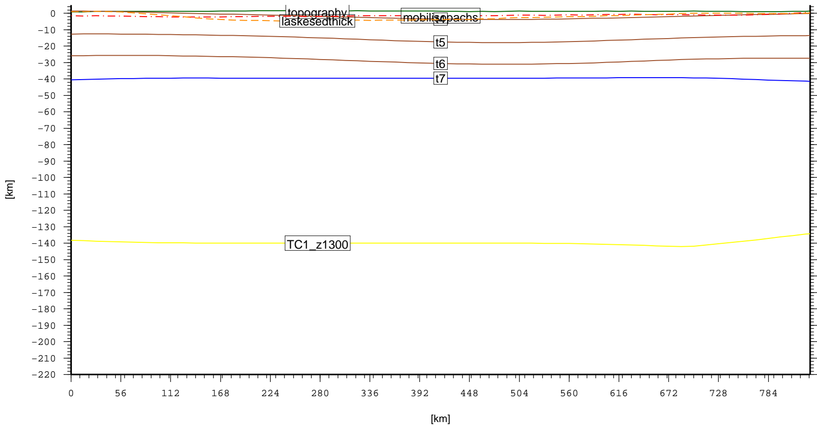
Cross section – CHN.Ordos_ShaanganningBasin (topo, laske sedthick, t4, t5, t6, t7)
