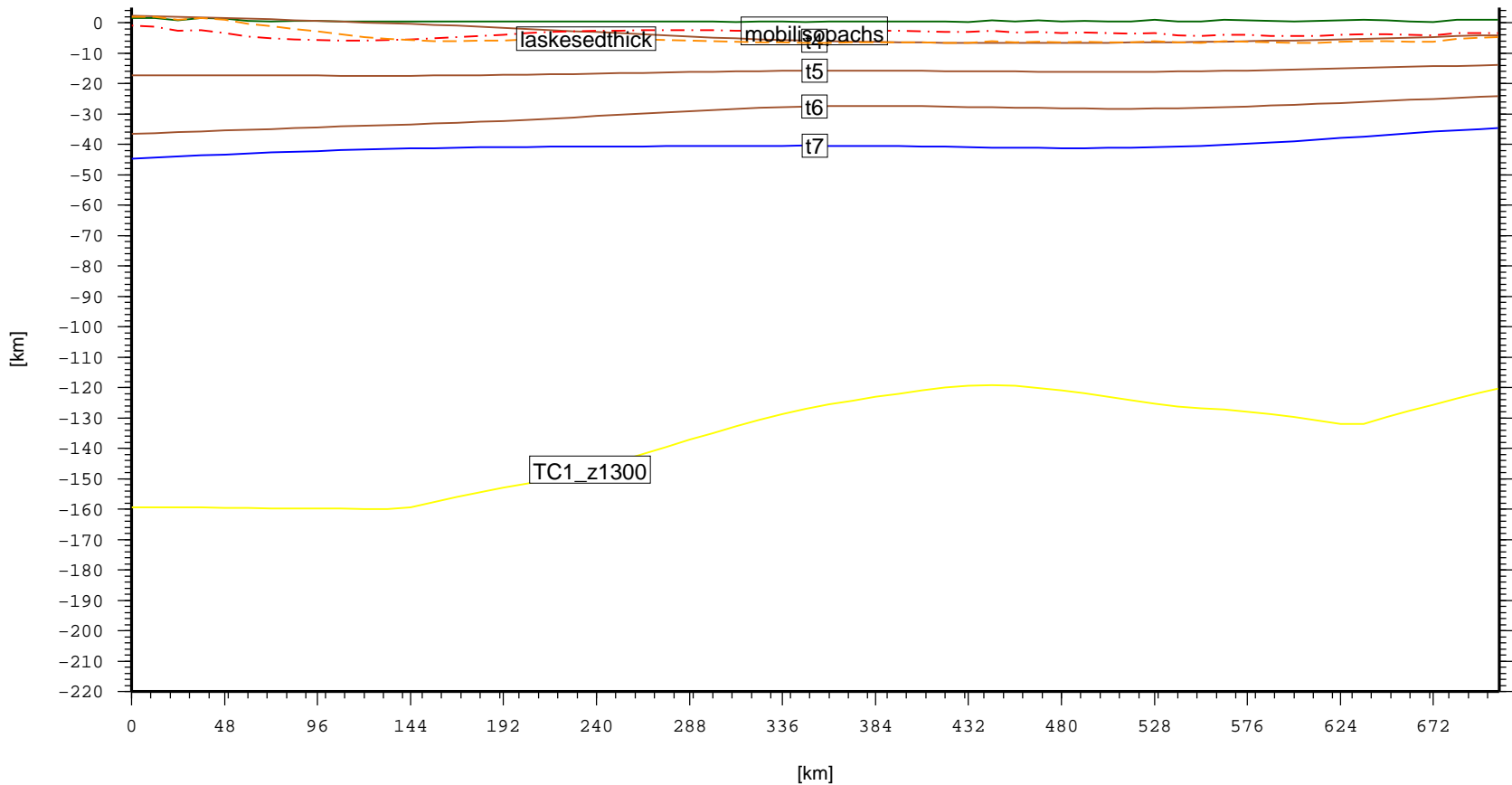
Cross section – CHN.Sichuan_SzechwanBasin (topo, laske sedthick, t4, t5, t6, t7)
