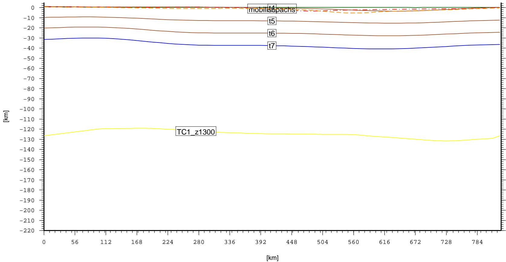
Cross section – CHN.SongliaoBasin (topo, laske sedthick, t4, t5, t6, t7)
