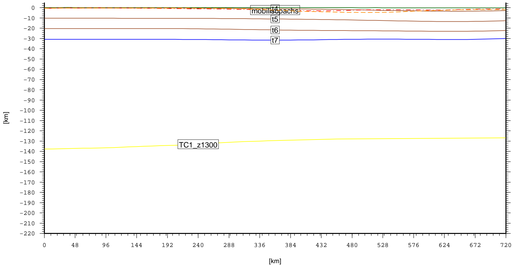
Cross section – CHN.SouthHuanghai_YellowSeaBasin (topo, laske sedthick, t4, t5, t6, t7)
