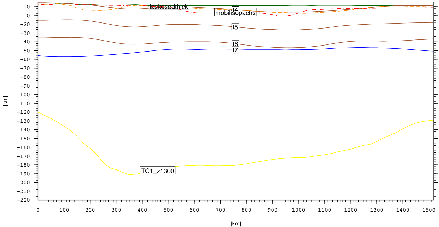
Cross section – CHN.Tarim_TalimuBasin (topo, laske sedthick, t4, t5, t6, t7)
