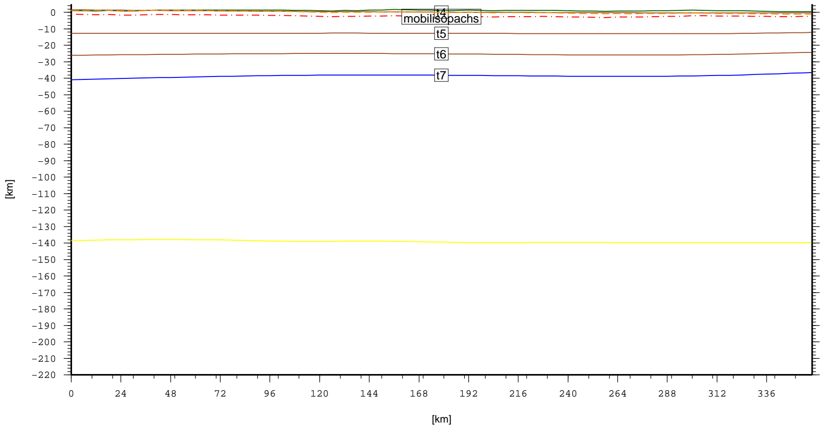
Cross section – CHN.WeihHeBasin (topo, laske sedthick, t4, t5, t6, t7)
