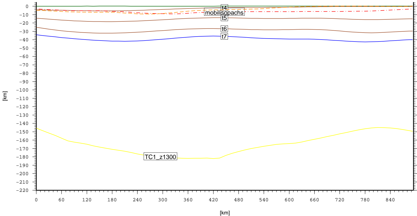
Cross section – EUR.Danish–PolishMarginalTrough (topo, laske sedthick, t4, t5, t6, t7)
