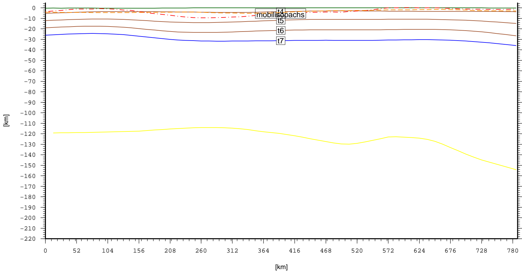
Cross section – EUR.FennoscandianBorderZone (topo, laske sedthick, t4, t5, t6, t7)
