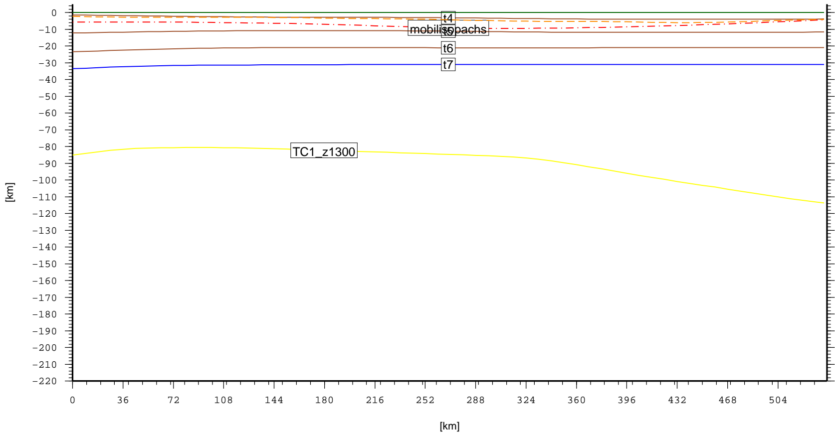
Cross section – EUR.NorthwestGermanBasin (topo, laske sedthick, t4, t5, t6, t7)
