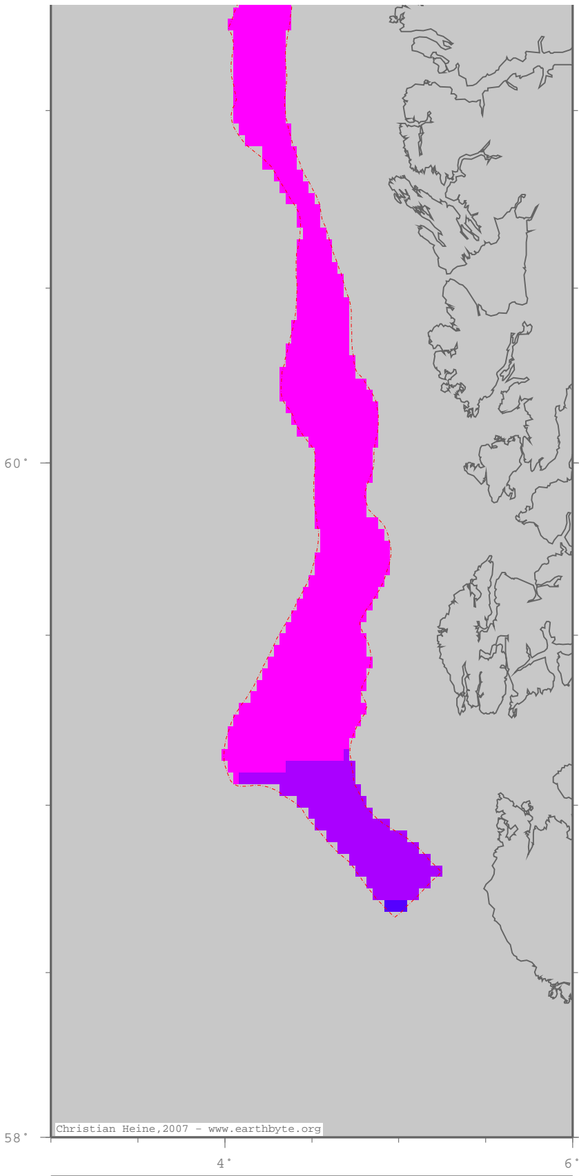
Crustal extension factor
