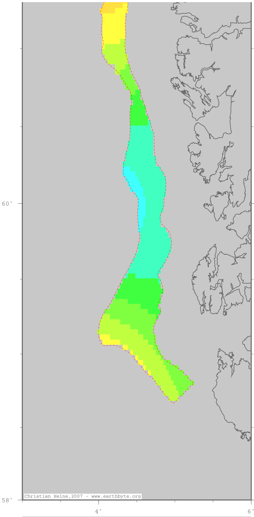
Total tectonic subsidence
