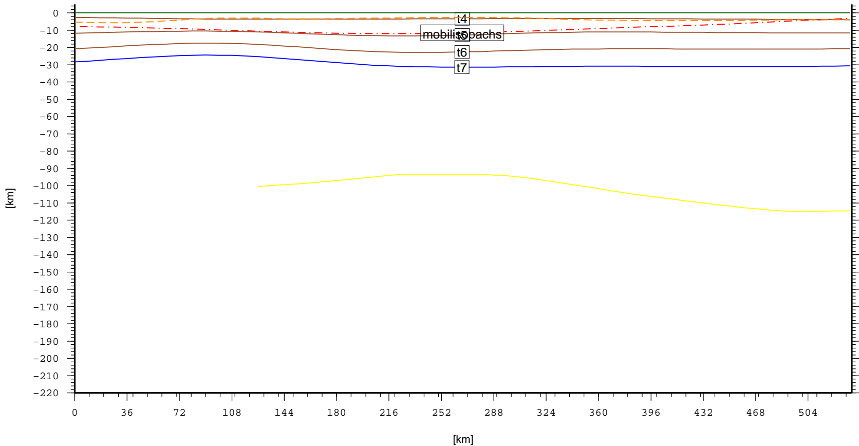
Cross section – EUR.Ringkobing–FynHigh (topo, laske sedthick, t4, t5, t6, t7)
