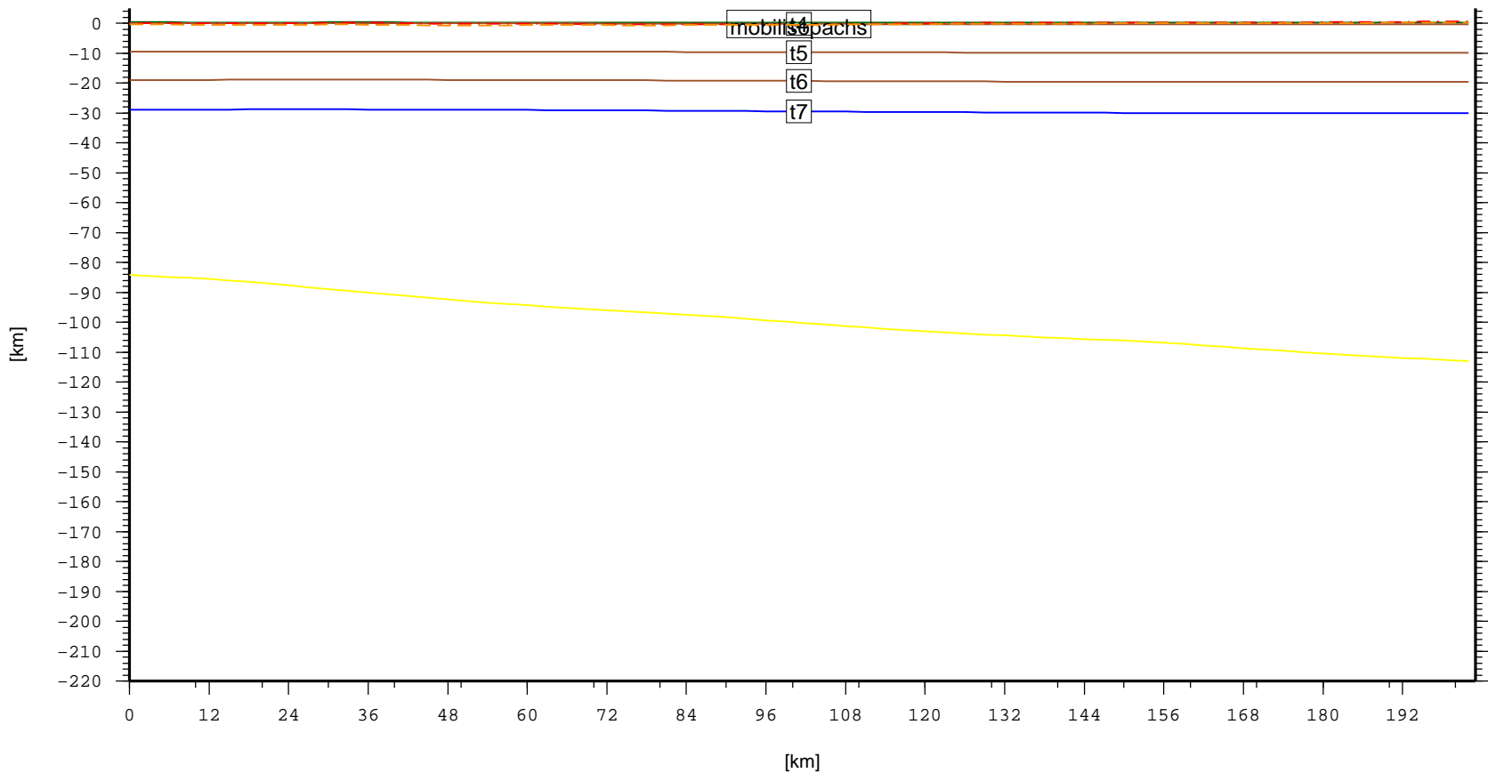
Cross section – EUR.ThuringianBasin (topo, laske sedthick, t4, t5, t6, t7)
