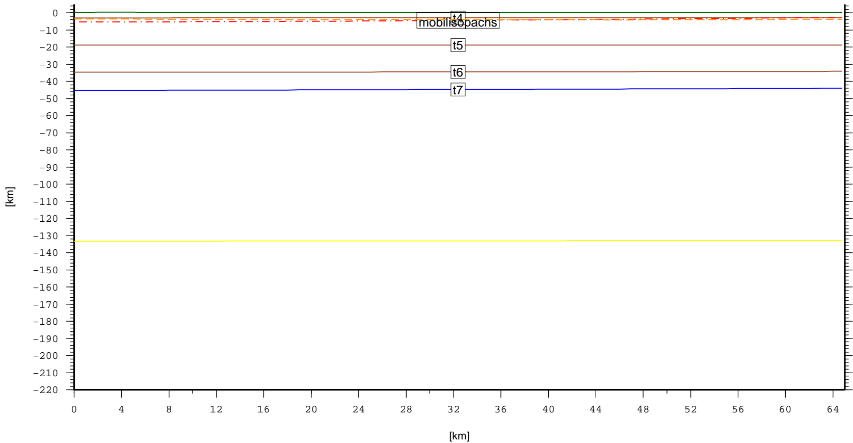
Cross section – NAM.ArdmoreandShermanBasinsMariettaSyncline (topo, laske sedthick, t4, t5, t6, t7)
