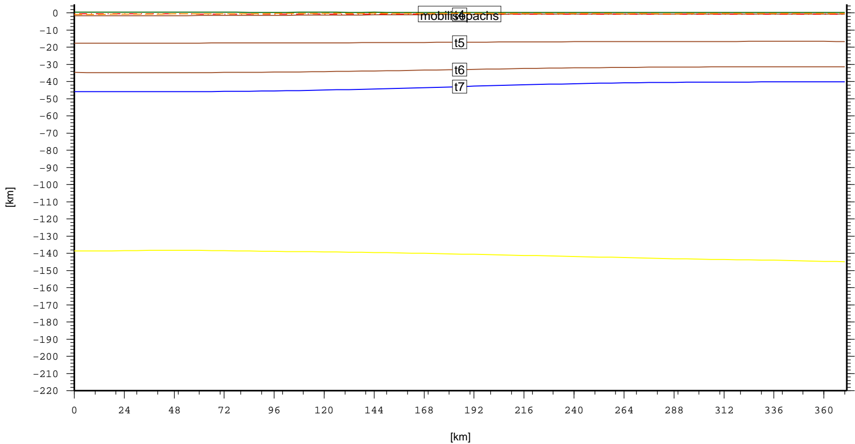
Cross section – NAM.ForestCityBasin (topo, laske sedthick, t4, t5, t6, t7)
