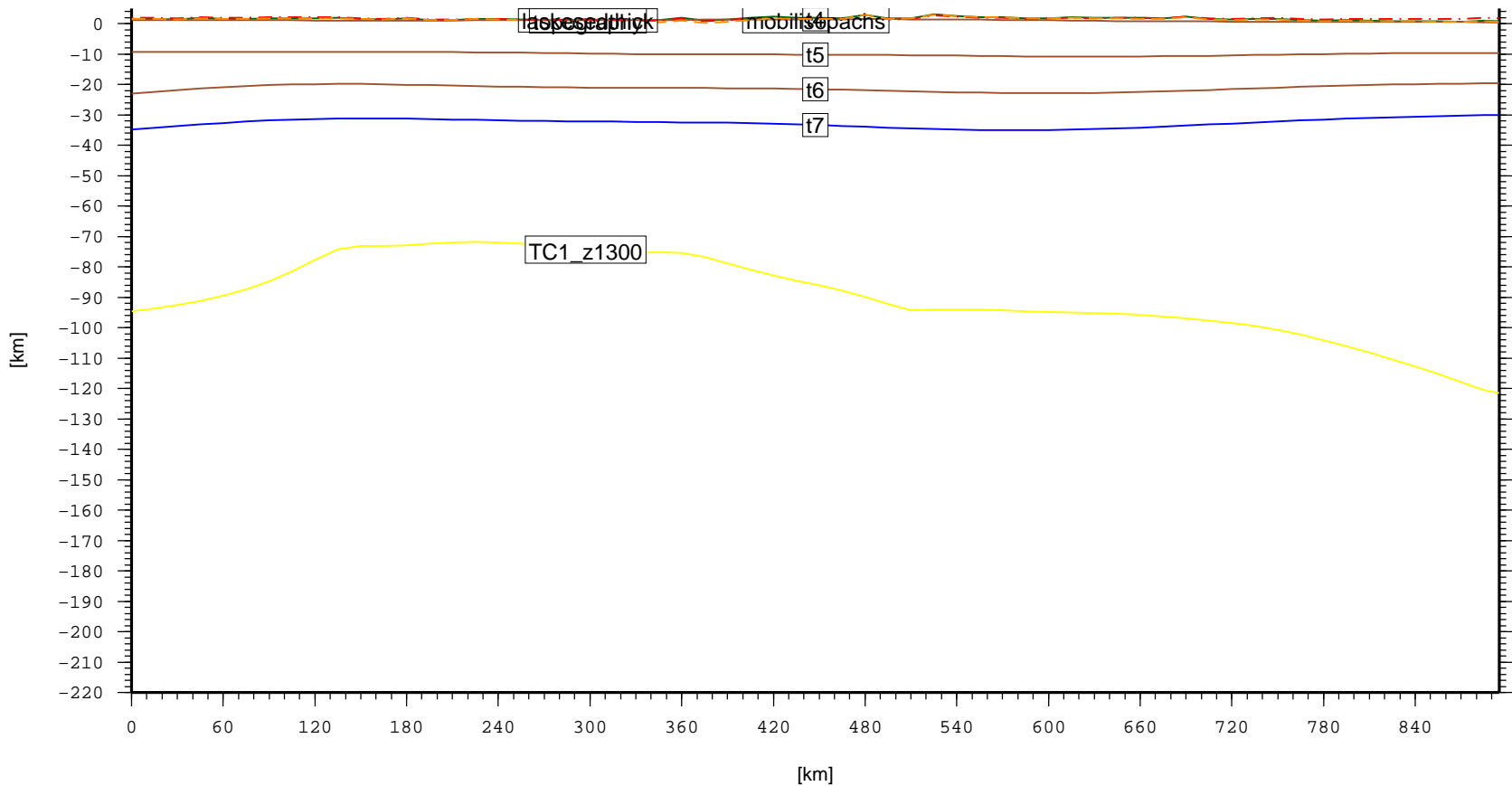
Cross section – NAM.GreatBasin (topo, laske sedthick, t4, t5, t6, t7)
