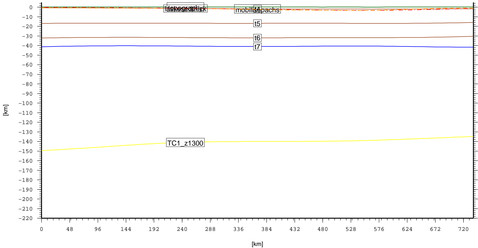
Cross section – NAM.IllinoisBasin (topo, laske sedthick, t4, t5, t6, t7)
