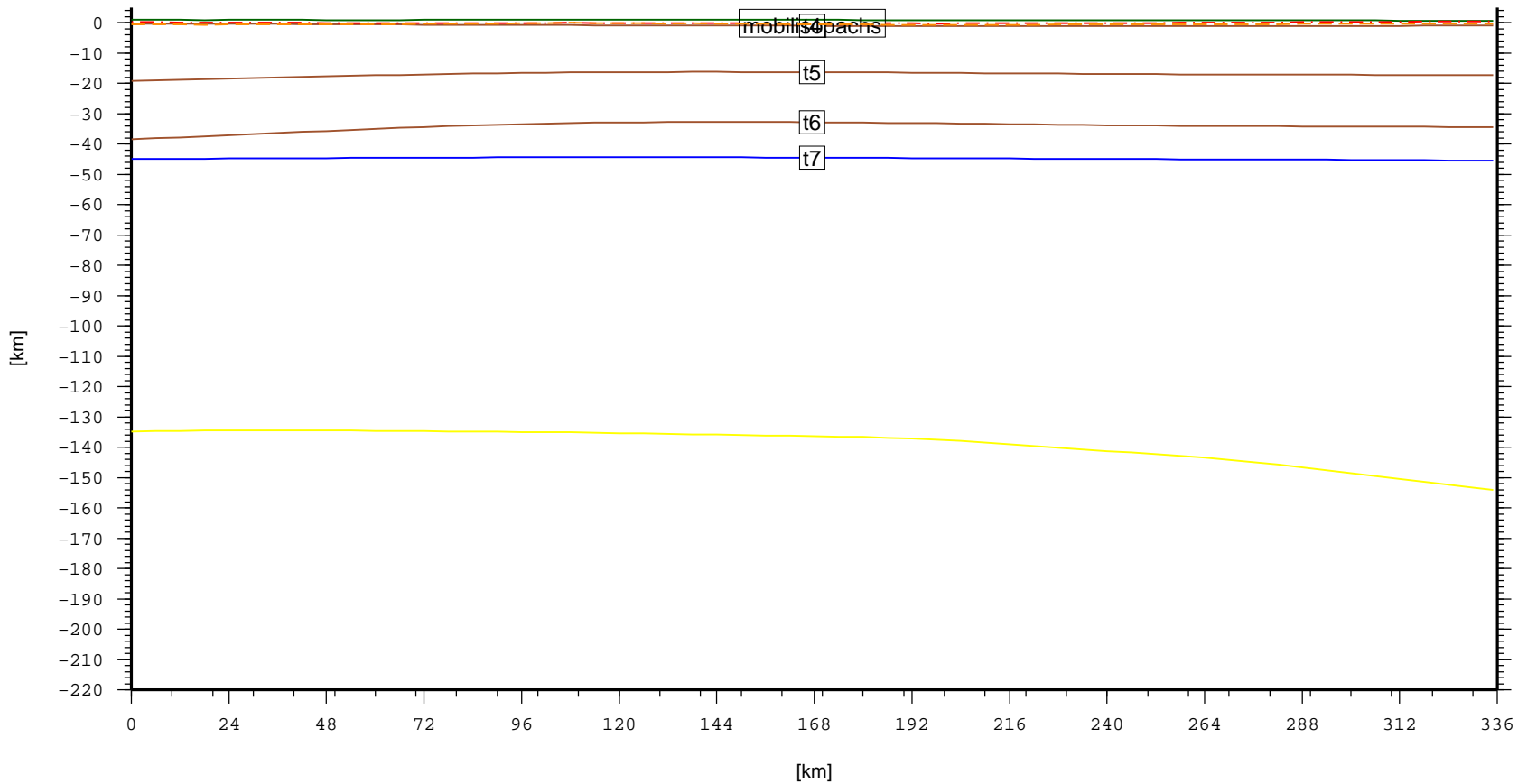
Cross section – NAM.KennedyBasin (topo, laske sedthick, t4, t5, t6, t7)
