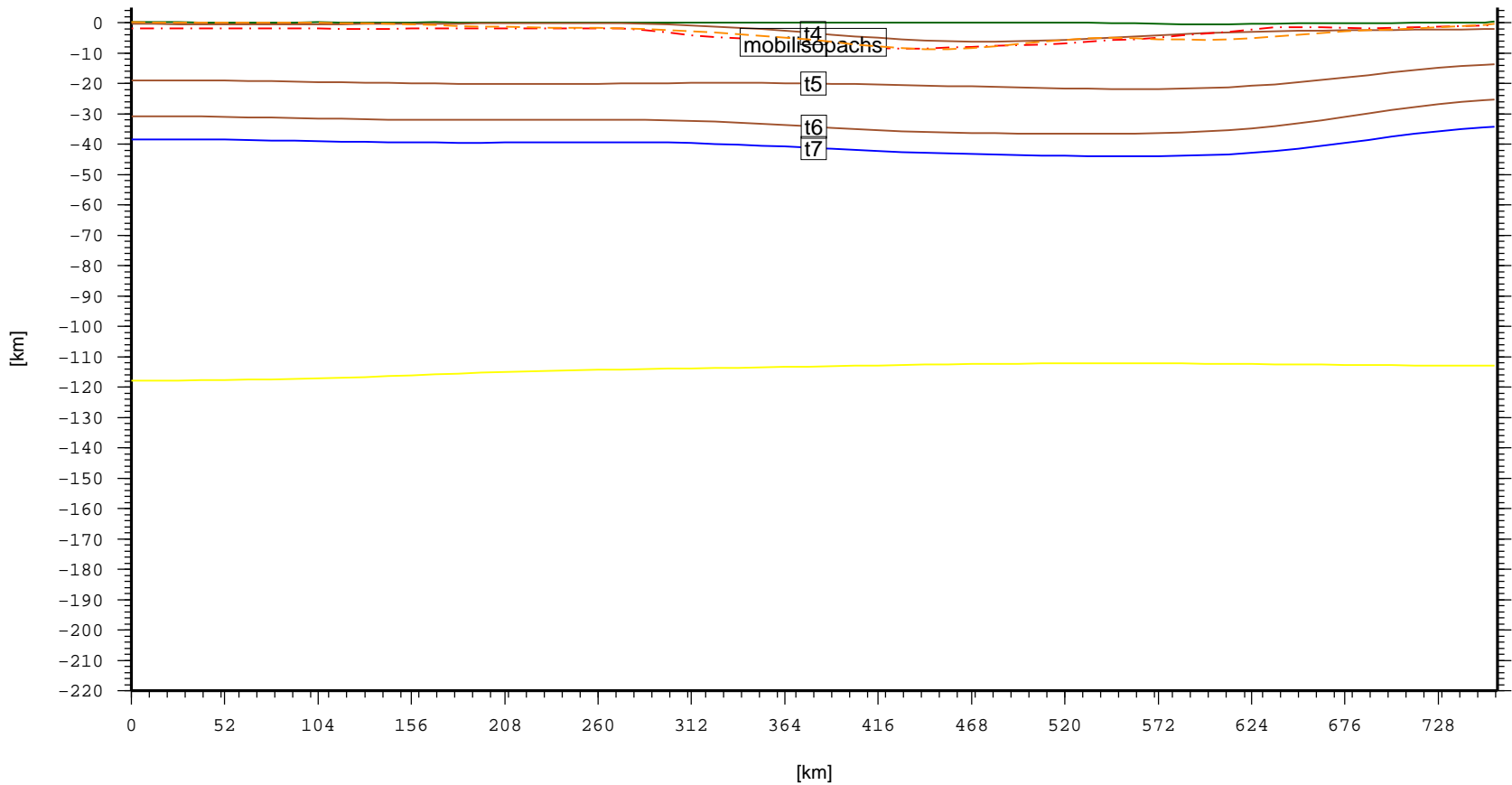
Cross section – NAM.MaritimesBasin (topo, laske sedthick, t4, t5, t6, t7)
