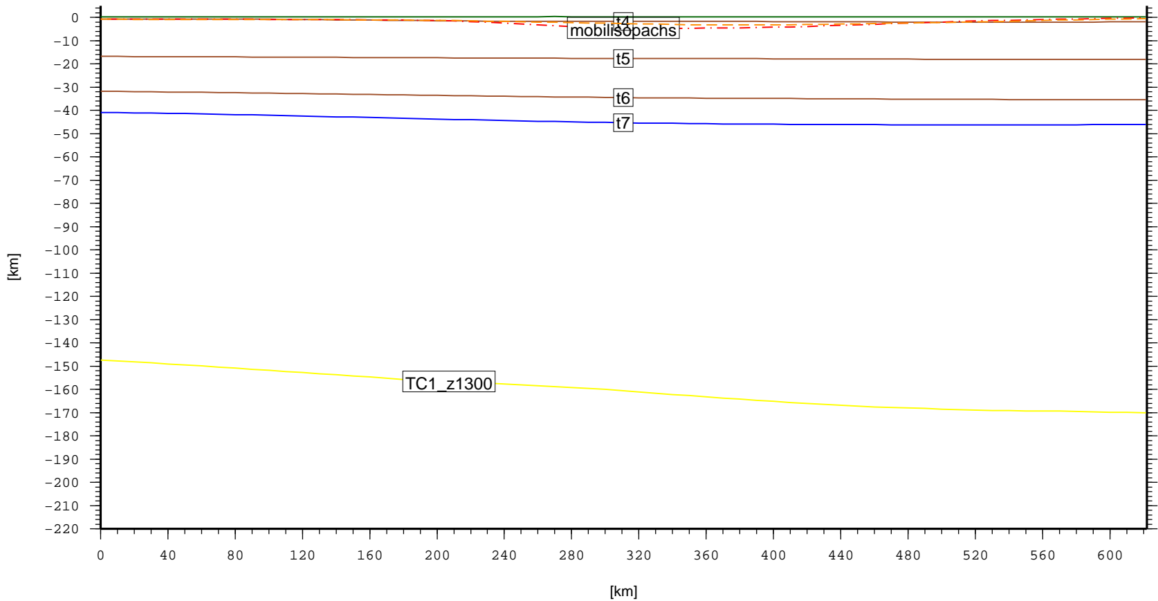
Cross section – NAM.MichiganBasin (topo, laske sedthick, t4, t5, t6, t7)
