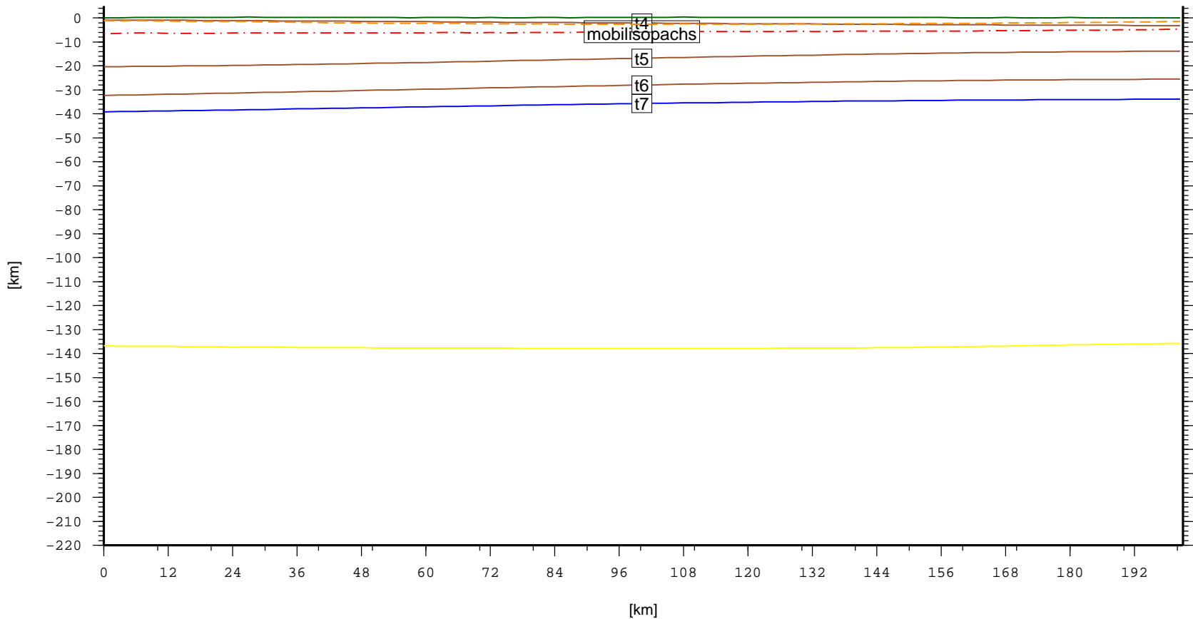
Cross section – NAM.NewarkBasin (topo, laske sedthick, t4, t5, t6, t7)
