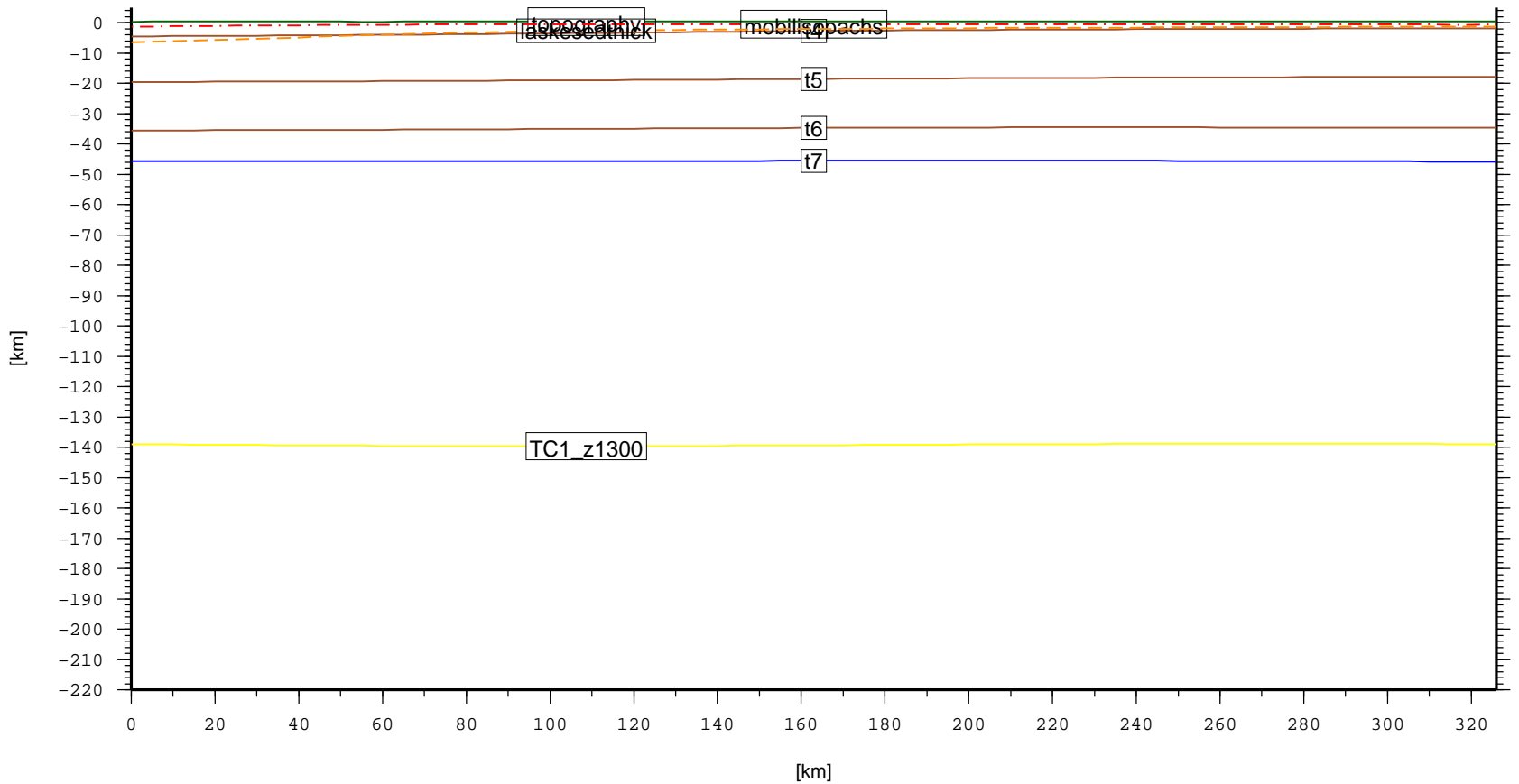
Cross section – NAM.SedgwickBasin (topo, laske sedthick, t4, t5, t6, t7)
